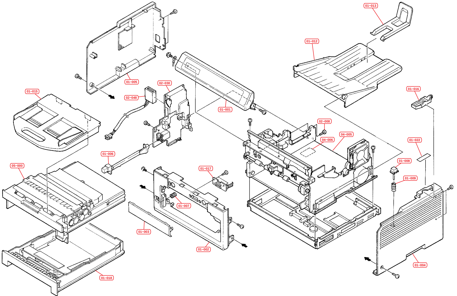
Fig.1 – Covers
