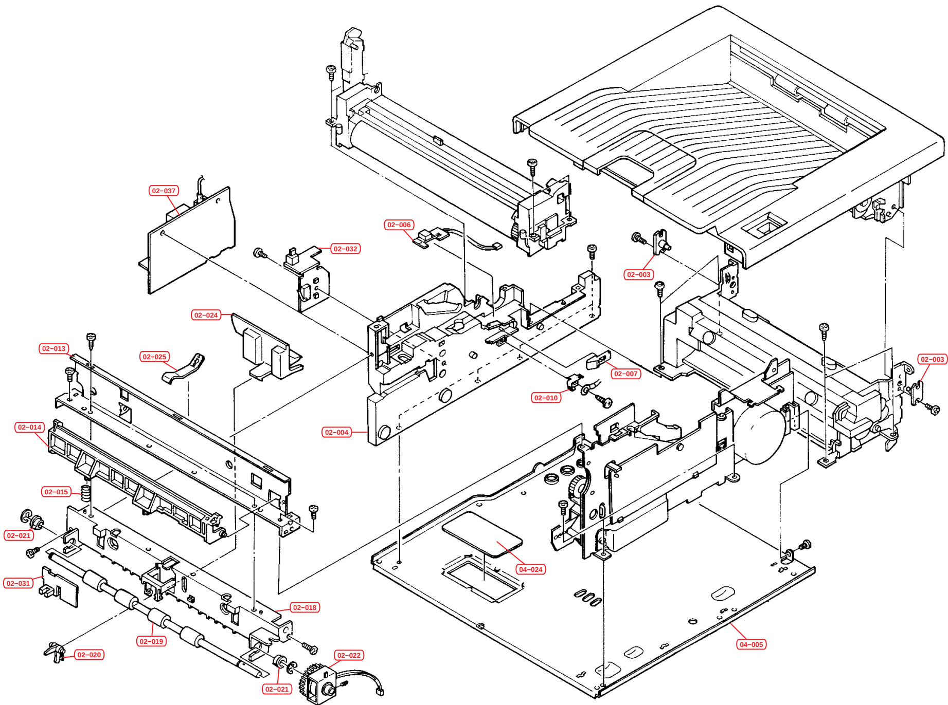
Fig.2 – Frame Unit
